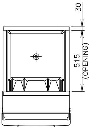
BIN TOP VIEW
